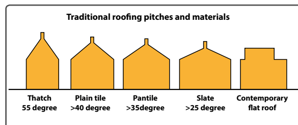
Fig 3.8.2 Roof pitches
