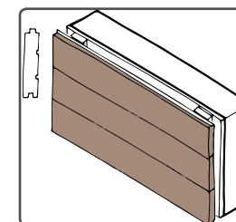
TONGUE & GROOVE - These produce a uniform look that suits contemporary houses. They have a flat face and in the absence of any overlapping, rain is kept out by the way the groove covers the tongue of the board below
