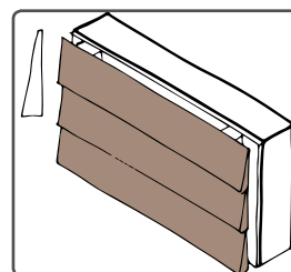
FEATHER EDGE - Boards are tapered across their width. This style of board produces a rustic, rural appearance that is perfect for more traditional homes, or barn style self builds
