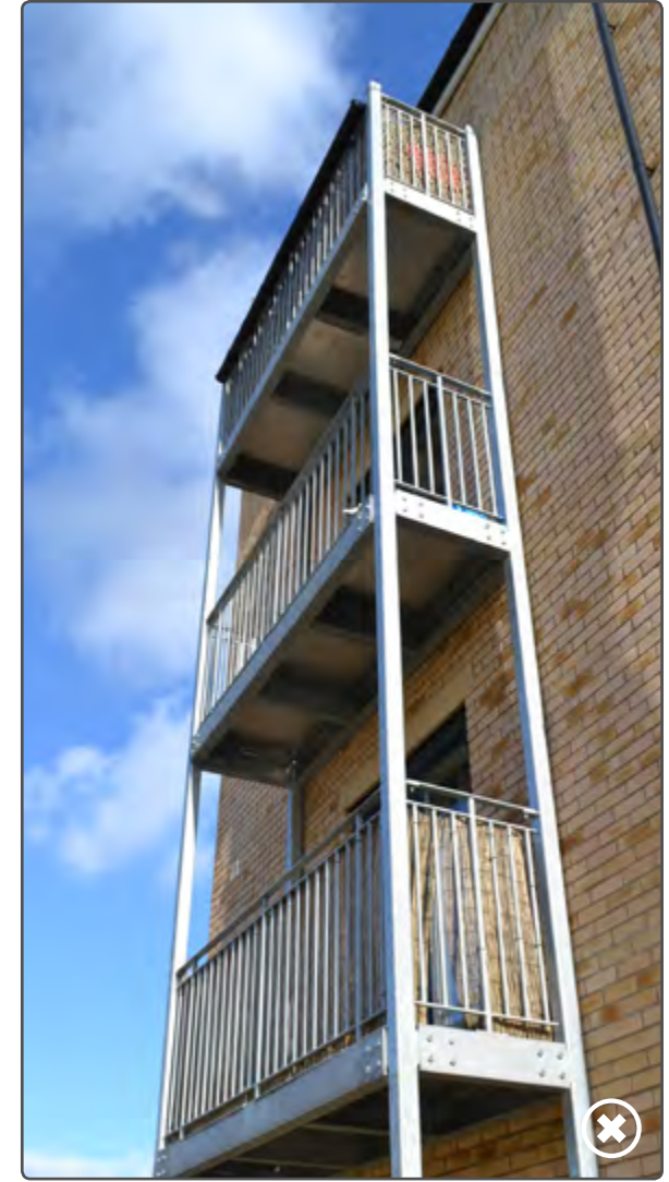
Poor external balcony design
