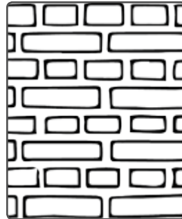
English bond
