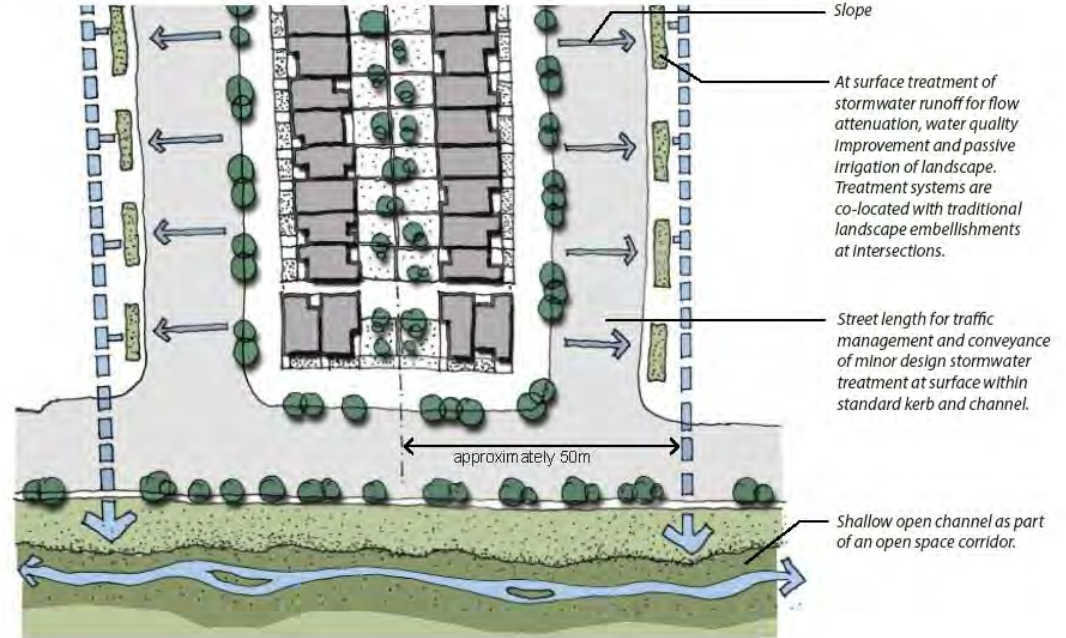
Figure 6.17 : Possible urban layout for a flat site
