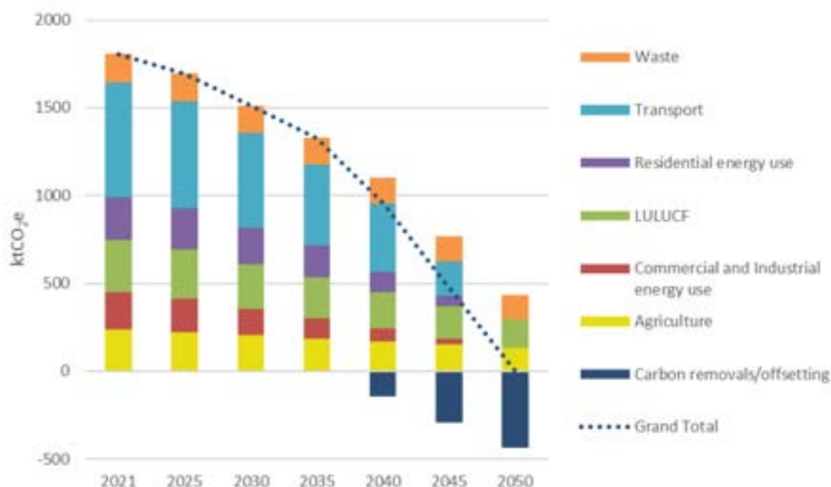
Figure 2.1 Huntingdonshire's decarbonisation trajectory in line with the Climate Change Committee's 'Balanced Pathway'
